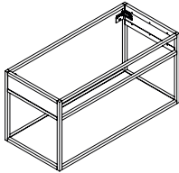
Wall structure 60cm | 80cm | 100cm | 120cm | 120cm DBL
